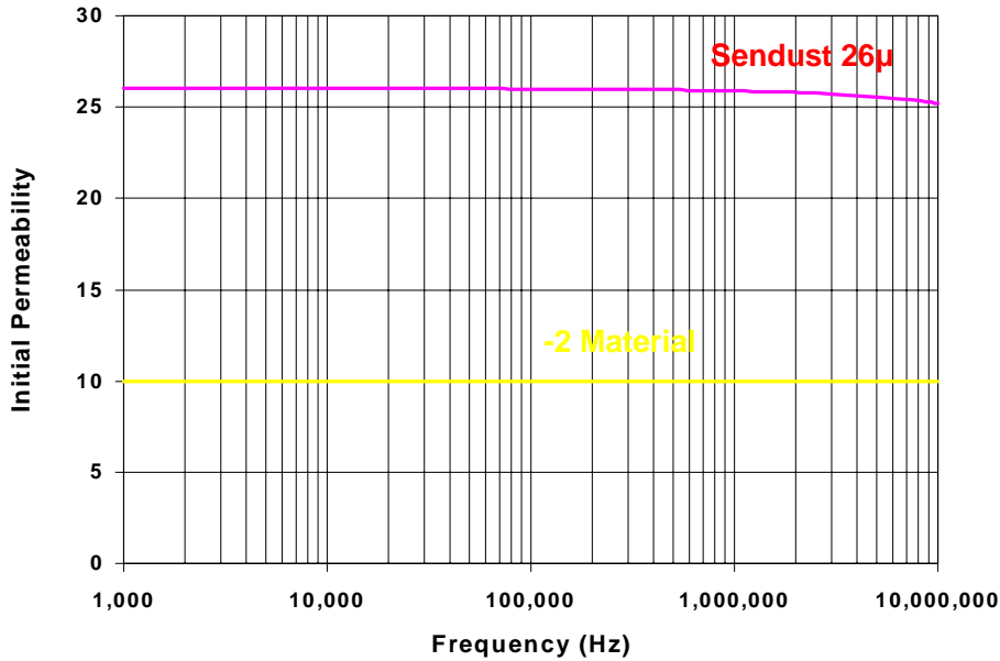
Figure 10: Initial Permeability vs. Frequency
