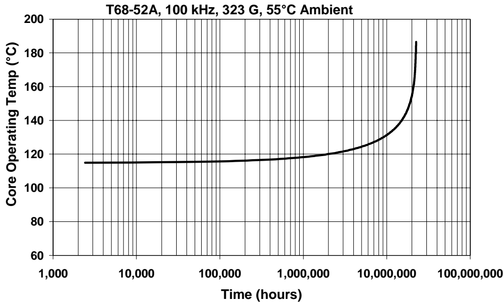
Figure 14: Core Operating Temperature vs. Time
