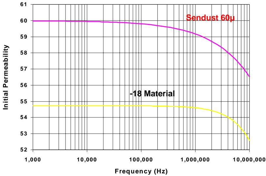
Figure 9: Initial Permeability vs. Frequency
