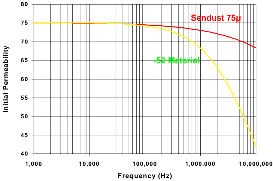
Figure 8: Initial Permeability vs. Frequency
