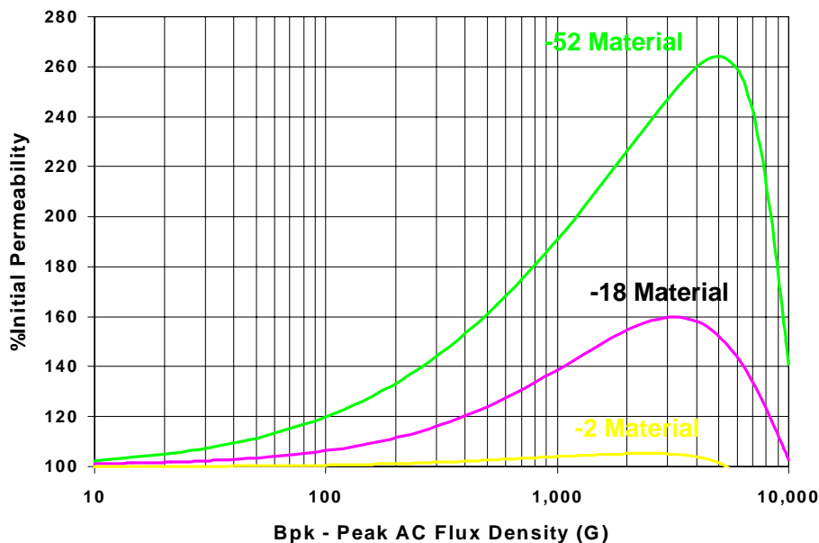
Figure 4: %Initial Permeability vs. Bpk
