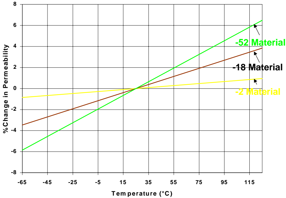
Figure 12: %Change in Permeability vs. Temperature – Iron Powder
