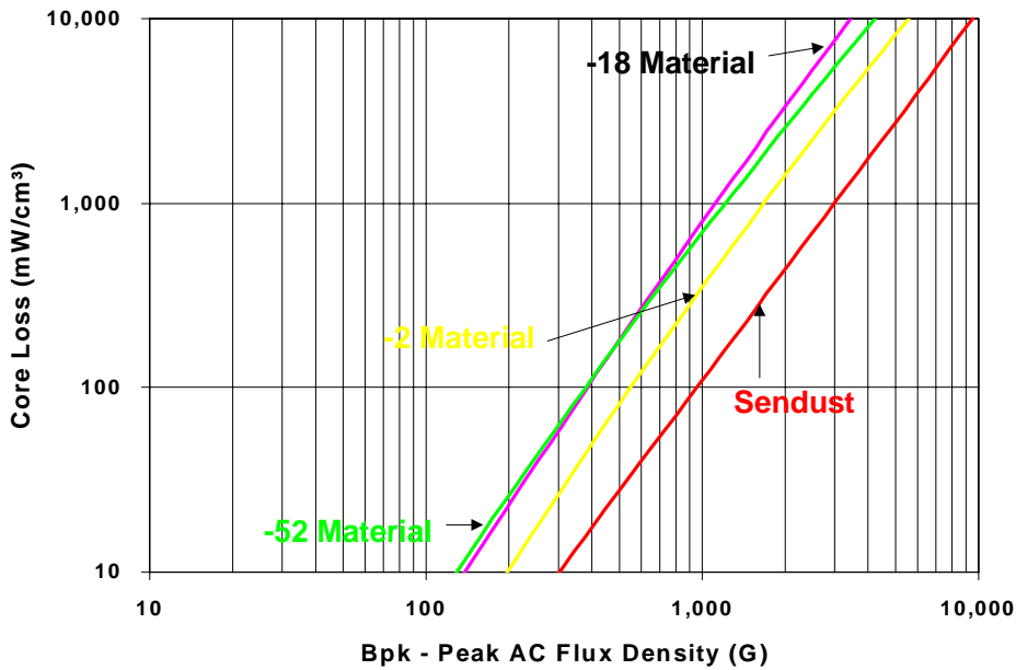
Figure 5: Core Loss vs. Bpk – 25 kHz
