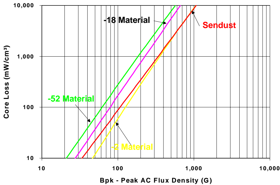
Figure 7: Core Loss vs. Bpk – 500 kHz
