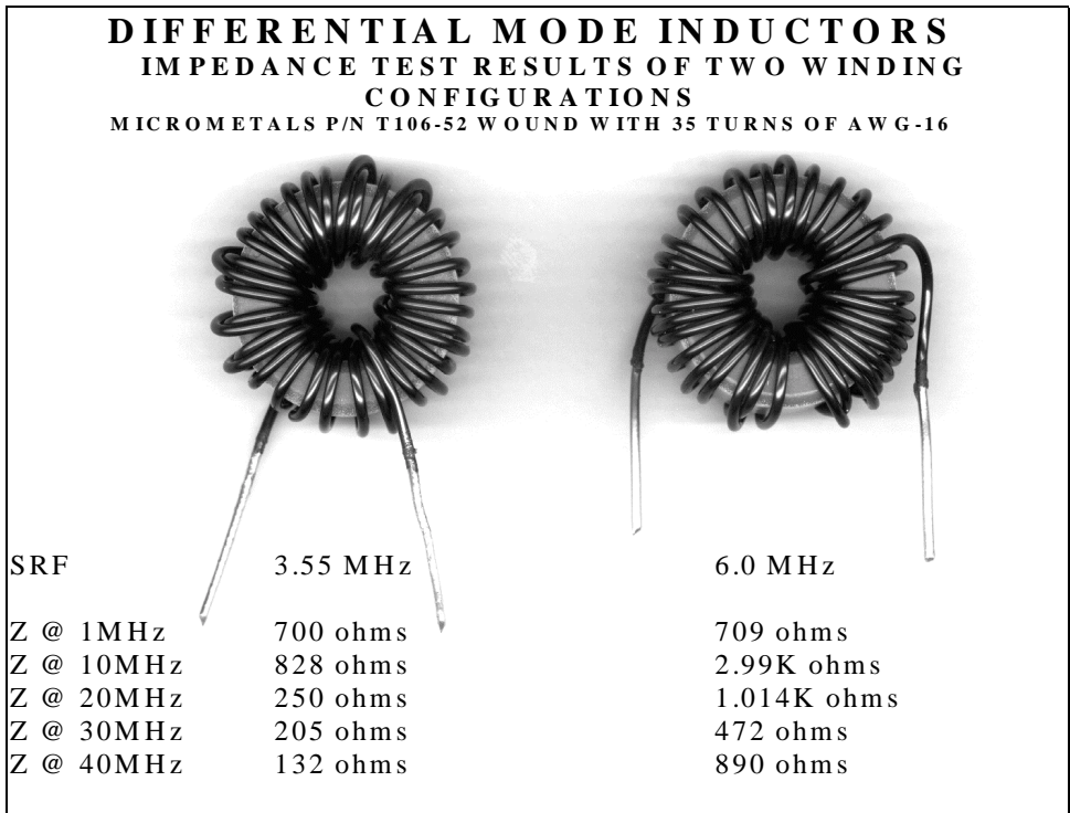
Figure 13: Differential Mode Inductor Winding Types
