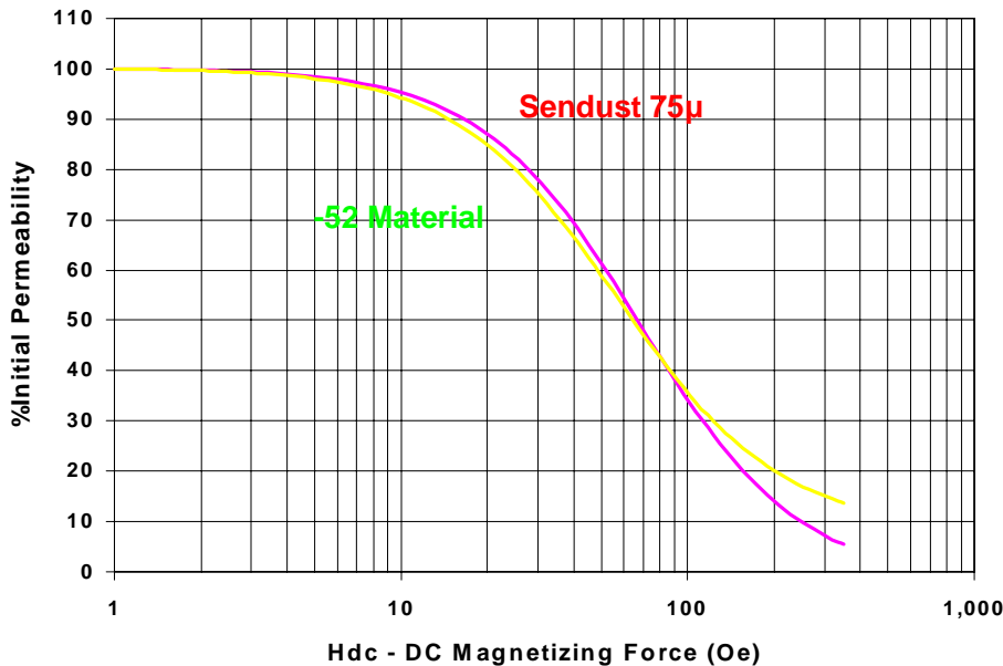
Figure 1: %Initial Permeability vs. Hdc
