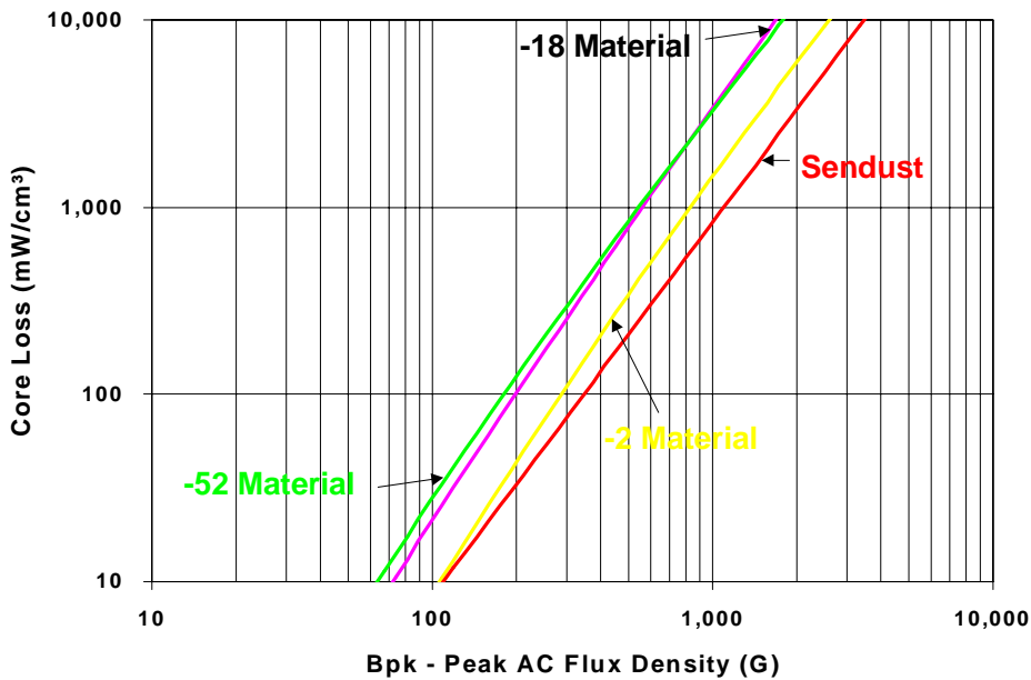
Figure 6: Core Loss vs. Bpk – 100 kHz
