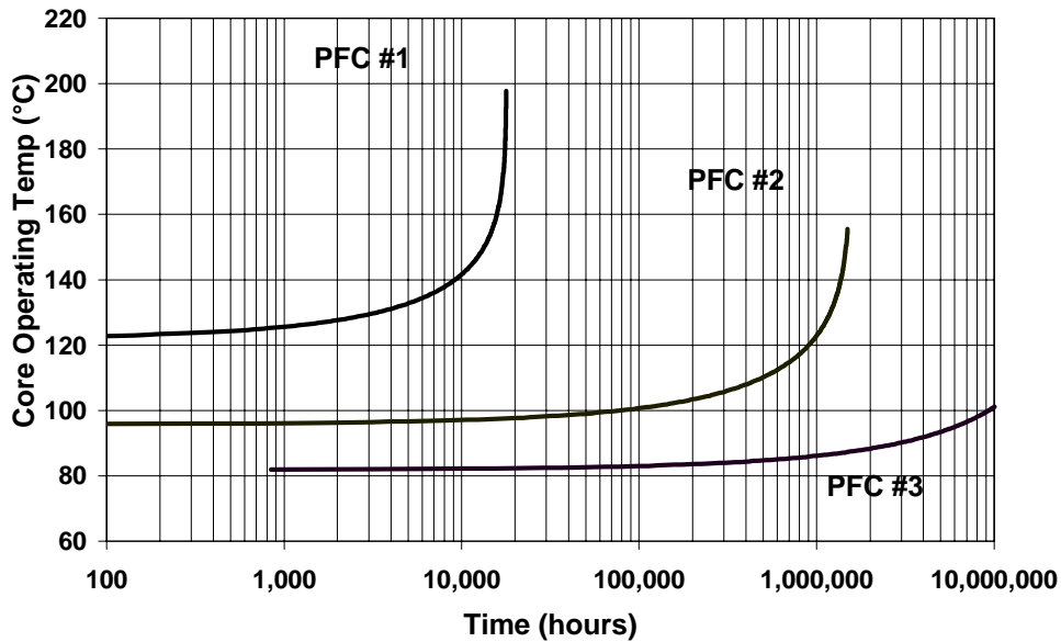
Figure 16: Core Operating Temperature vs. Time – PFC Designs
