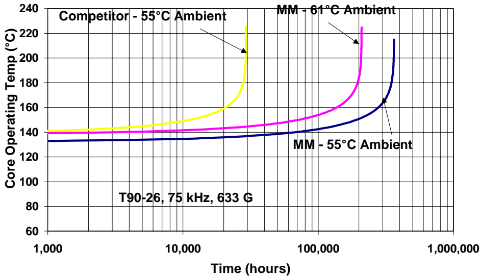
Figure 15: Core Operating Temperature vs. Time
