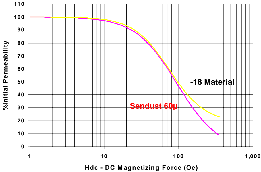
Figure 2: %Initial Permeability vs. H dc
